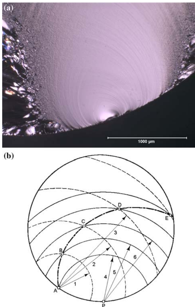
Fig. 5 Appearance and construction of a Wallner line. a Fused silica glass rod, broken in tension, showing Wallner lines and mirror markings (Courtesy of G.D. Quinn, NIST, Gaithersburgh, USA). b Construction scheme (Ref. University of Freiburg, Freiburg i.B., Germany). A —starting point of the ultrasound wave; 1–3 —circular arcs of the ultrasound wave at three time periods; P —starting point of fracture; 4–5 —fracture front radii at three time periods; intersecting points B–E —Wallner line
