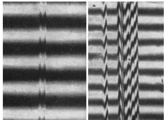
Fig. 8 Micro-plasticity in PMMA (interference microscope images, magnification 920:1, diamond tip 8 g). Left quartz glass with network structure and strong principal valency bond; right PMMA with chain structure and weak secondary valency bond [43]
