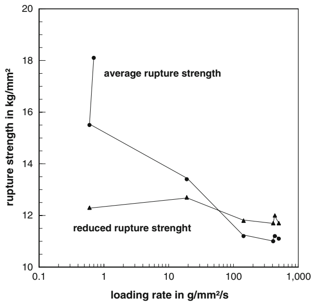
Fig. 4 Stress-thermal fracture, evidenced due to the dependence of the average rupture strength on loading rate. The reduced rupture strength , however, does not depend on loading rate, but is a material parameter. Temperature 400–445 °C. Measurements taken from Eichler [13]
