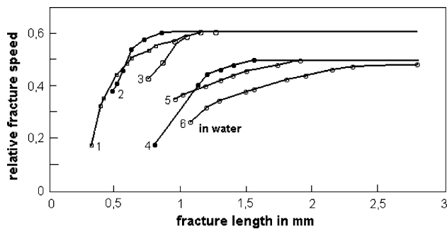
Fig. 7 Fracture propagation velocities in glasses as functions of loading rate and environment [19]. 1 Quartz glass 3.45 kg/mm 2 , 2 quartz glass 4.47 kg/mm 3 , 3 quartz glass 4.17 kg/mm 2 , 4 optical glass 2.94 kg/mm 2 , 5 optical glass 3.25 kg/mm 2 , 6 optical glass 2.70 kg/mm 2 (in water)
