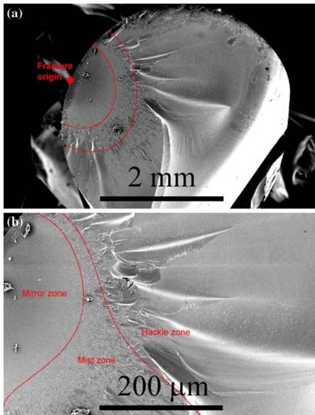
Fig. 2 Fracture surface of a glass rod broken during a tensile test. a General view with fracture origin; b topographical features (Photographies: University of Cambridge, Cambridge, UK)
