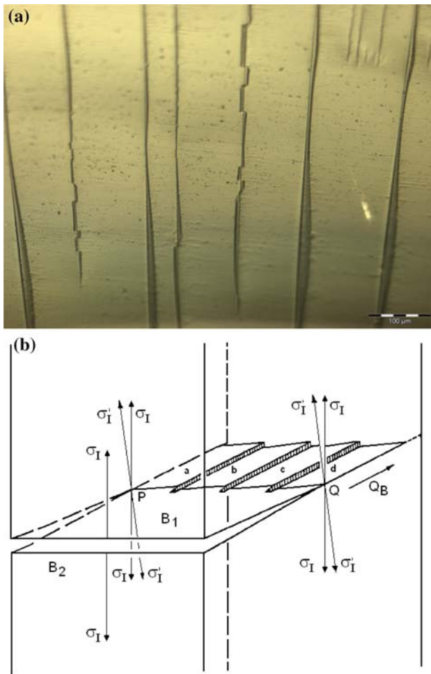
Fig. 6 a Fracture lances, formed during ball indentation of a soda-lime glass sample. Scale bar: 100 μm (Photograph: Andreas Momber). b Scheme of fracture lance formation in a brittle solid (adapted from Kerkhof [27])
